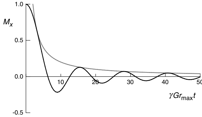
The black line shows the decay of magnetization due to the action of a gradient pulse. The grey line is an approximation, valid at long times, for the envelope of the decay.
