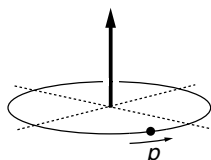
A mass going round a circular path possesses angular momentum, represented by a vector which points perpendicular to the plane of rotation.
