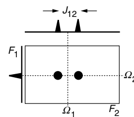
Schematic HMQC spectrum for two coupled spins.
