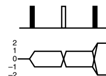
Pulse sequence for generating double-quantum coherence. Note that the 180^\circ pulse simply causes a change in the sign of the coherence order.
