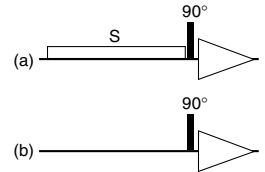
Pulse sequence for recording steady state NOE enhancements. Sequence (a) involves selective irradiation of the S spin leading to saturation. Sequence (b) is used to record the reference spectrum in which the intensities are unperturbed.
