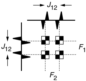
Schematic view of the diagonal peak from a COSY spectrum. The squares are supposed to indicate the two-dimensional double dispersion lineshape illustrated below
