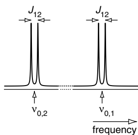
Fig. 2.5 Schematic spectrum of two coupled spins showing two doublets with equal splittings. As indicated by the dashed lines, the separation of the Larmor frequencies is much larger than the coupling between the spins.
