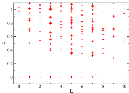
FIG. 2. Spectrum of the model Hamiltonian (1) for N_\uparrow + N_\downarrow = 4 + 4 on a sphere with N_\phi = 8 flux quanta, i.e., n = 2 flux quanta above the ground state as a function of total angular momentum L . The counting of quasihole states in the zero-energy manifold matches the theoretical prediction given in Eq. (18). We further identify the gap in this finite-size system to be \Delta_{N=8} \simeq 0.2812 .
