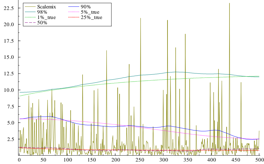
Figure 6: Absolute values of simulated series, true quantiles and random walk 98%, 90% and 50% quantiles fitted to simulated data by CV.
