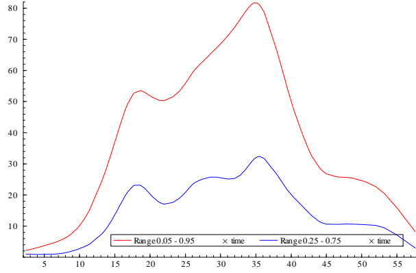
Figure 9: Motorcycle data: 75-25 and the 95-5 inter-expectile ranges.
