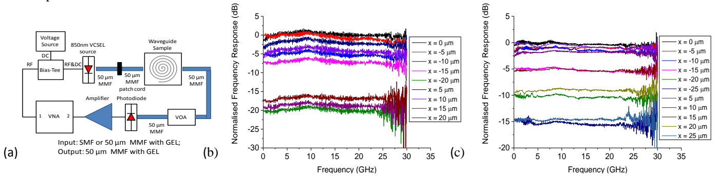
Fig. 1. (a) Experiment set-up of S_{21} parameter measurement; (b) and (c) are normalised frequency response of the spiral waveguide for different horizontal offsets under a SMF and 50 \mu\text{m} MMF input, respectively.
