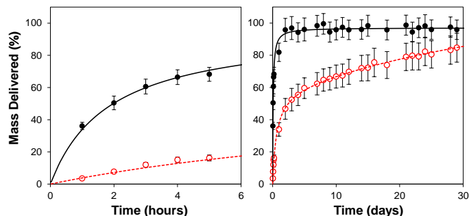
Figure 2. (left) Calcein release during the first 5 hours and (right) 30 days from UiO-66, black closed circles, and a_m\text{UiO-66} , red open circles. Black solid and red dotted lines represent the kinetics of delivery, fitted using non-linear regression on UiO-66 and a_m\text{UiO-66} , respectively.
