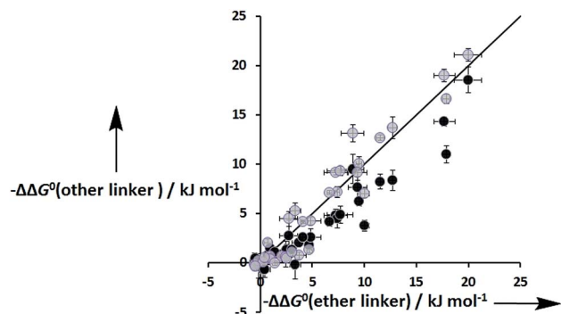
Fig. 8 Total free energy contribution due to intra-molecular H-bonding for ligands with an ether linker, \Delta\Delta G^0 (ether linker), compared with data for the corresponding ligands with an ester linker (black) and aromatic linker (grey), \Delta\Delta G^0 (other linker). The line corresponds to \Delta\Delta G^0 (other linker) = \Delta\Delta G^0 (ether linker).
