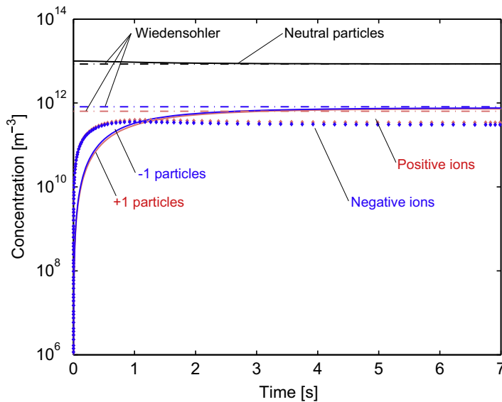
Fig. 4. Typical neutraliser temporal charging curve for positive, negative and neutral particles. Specific model constants are D_p = 15 \text{ nm} , N_{\text{tot}} = 10^{13} / \text{m}^3 , q = 10^{12} / \text{m}^3 / \text{s} , Wiedensohler ions.
