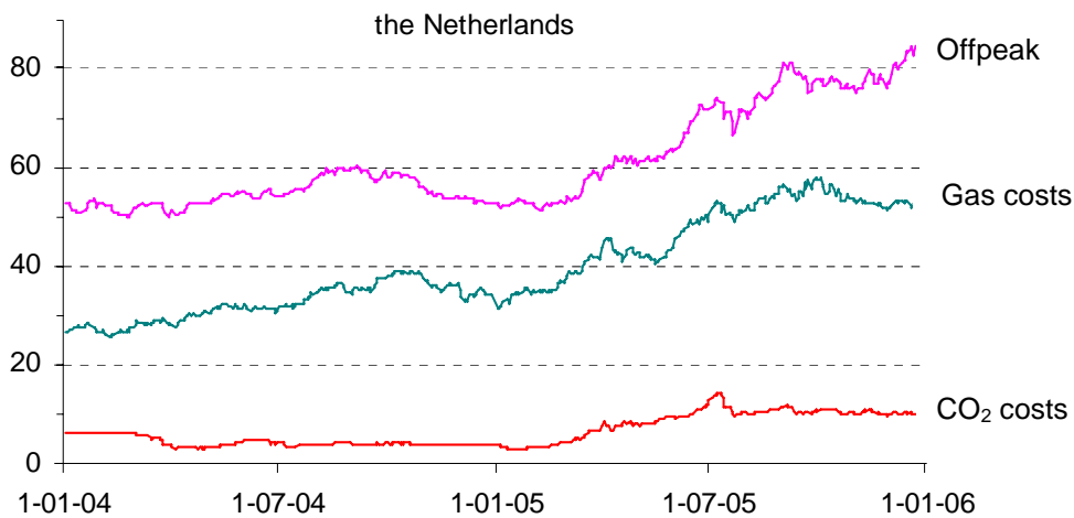
Figure 4 Peak power prices versus fuel/CO 2 costs in the Netherlands (year ahead, 2004-2005)
