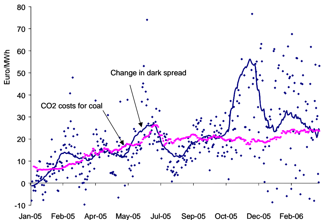
Figure 8 Coal price corrected price increase for electricity (3-4 pm) depicted as dots and their 40day moving average (volatile line) and the evolution of the CO 2 price
