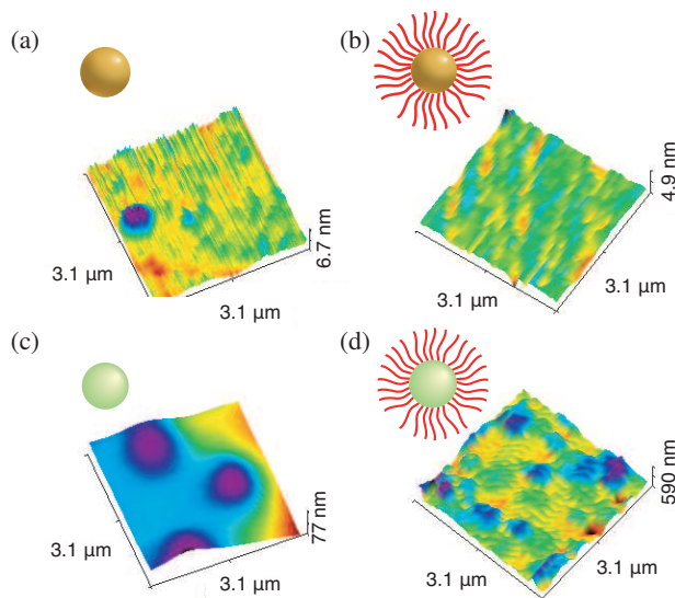
Figure 3. AFM topographical measurements of a) Au-NP 3a , b) Au CP-NP hybrid 3b , c) CdSe-NP 5a , d) CdSe CP-NP nanohybrid 5b .
