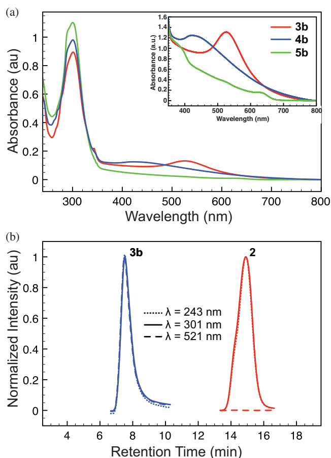
Figure 1. a) UV-Vis Spectroscopy of CP-NP nanohybrids 3b , 4b and 5b . b) GPC analyses of thiol-functional polymer 2 and CP-NP nanohybrid 3b in THF. There is a perfect overlay of the absorbance from the polymer ( \lambda_{\text{max}} = 243 and 301) and the NP ( \lambda_{\text{max}} = 521 ) in CP-NP nanohybrid 3b , supporting covalent conjugation of the polymer to the NP.
