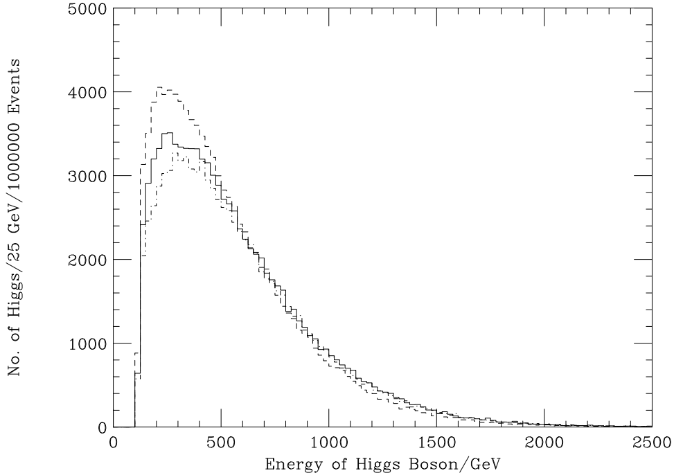
Figure 1: Parton-level energy spectra of Higgs bosons, m_H = 115 GeV. Solid: predicted energy spectrum of Higgs bosons from decay of black holes with initial masses 5.0-5.5 TeV. Dashed: neglecting time variation of temperature. Dot-dashed: neglecting grey-body factors.
